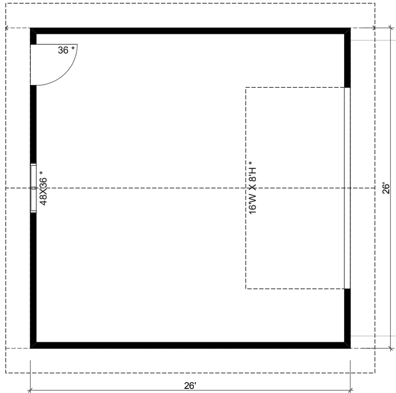
1 | GARAGE PLAN
