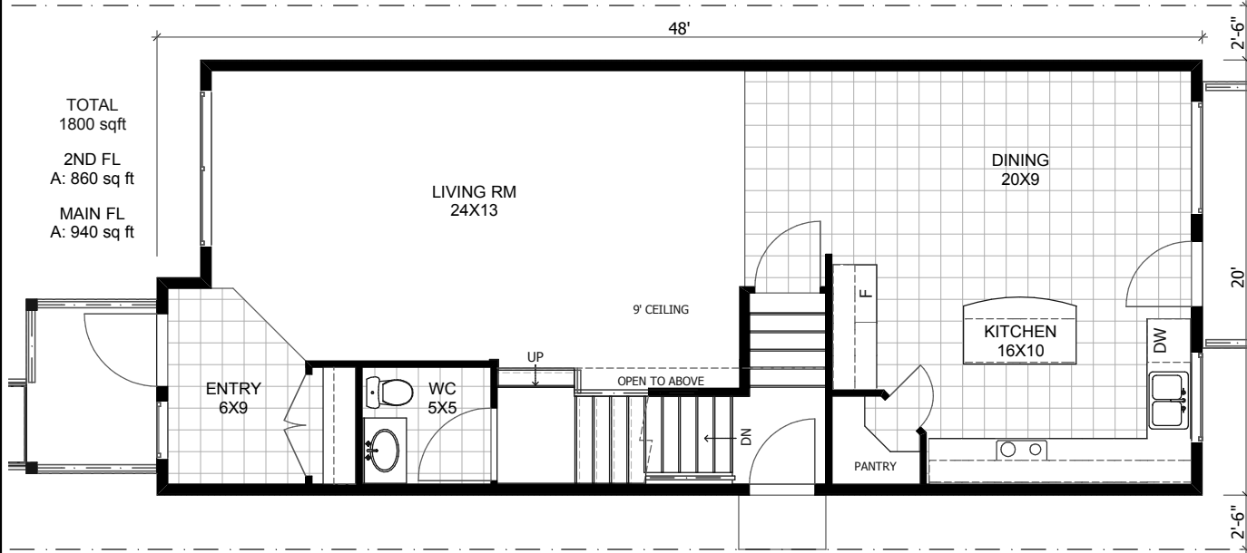
1 | MAIN FL PLAN
