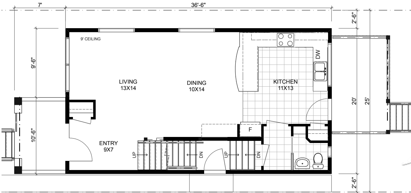
1 | MAIN FL PLAN SCALE 1/8" = 1'-0"
