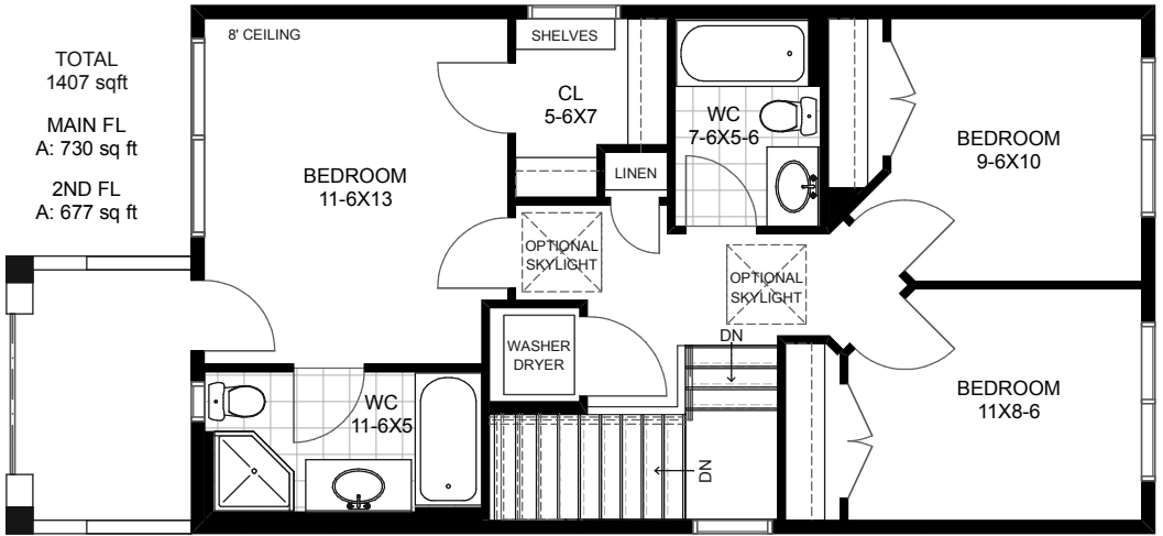
2 | 2ND FL PLAN SCALE 1/8" = 1'-0"
